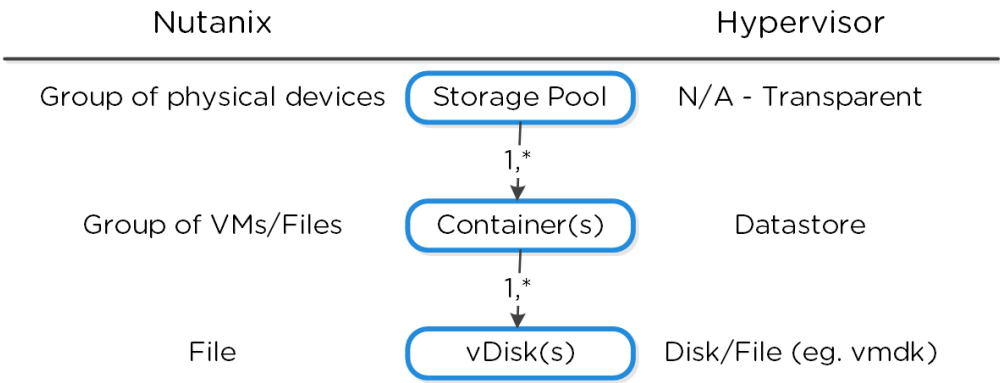
High-level Filesystem Breakdown
