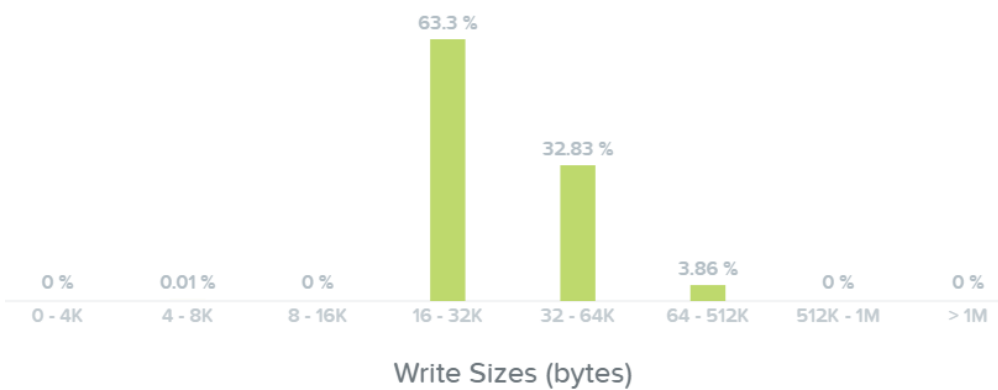
I/O Metrics - Write I/O Size histogram
