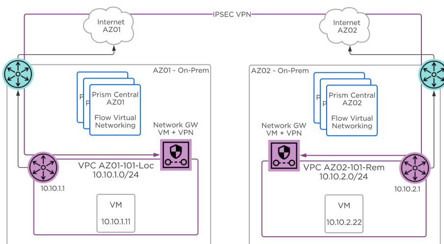
Flow Virtual Networking - Layer 3 VPN
