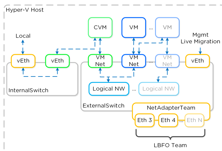
Hyper-V Virtual Switch Network Overview
